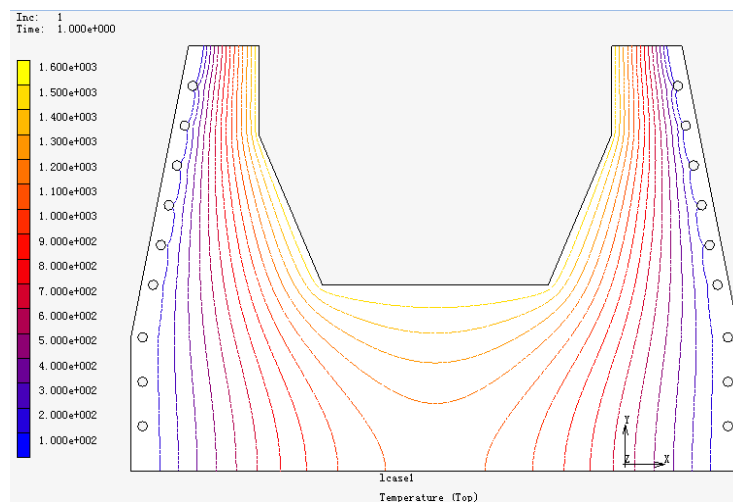
Fig. 6 The Temperature isoline of the hearth
