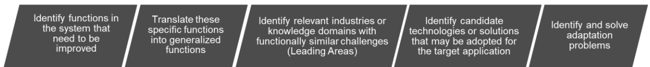
Fig. 9. FOS algorithm
