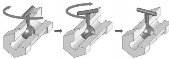
Fig. 12. Ball valve
