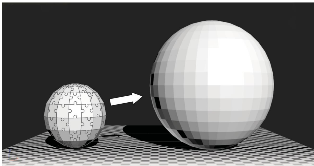
Fig. 2 Knowledge analogy
