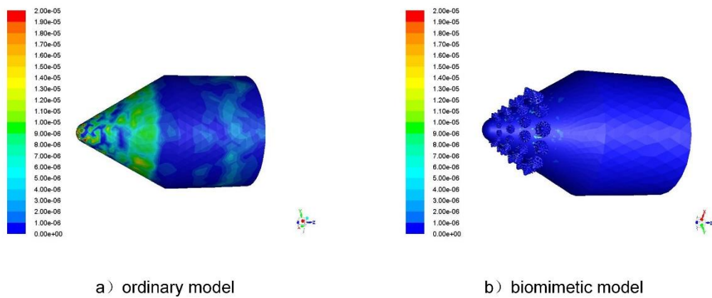
Fig. 7. Erosion rate
